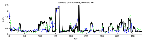
Fig. 2. Absolute error for GPS (bold black), BPF (solid blue) and PF (dashed green).
