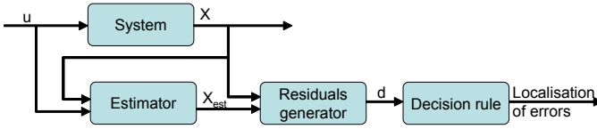
Figure 1. Block diagram of system monitoring
