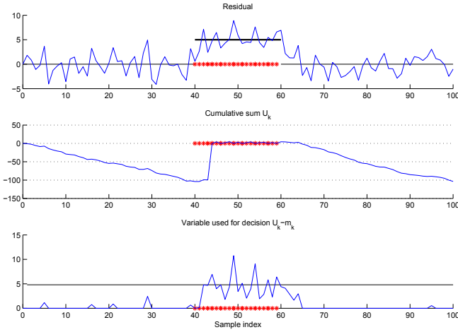
Figure 2. Illustrative example of Page's test. The signal to consider is plotted on the top graph. The corresponding cumulative sum and decision variable are beyond. The red stars denote the sample indexes for which the test has detected a mean change.
