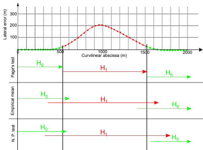
Figure 5. Sequential outcomes of three trend tests on hypotheses H_0 (correct road segment) and H_1 (erroneous road segment). The lateral distance to the map-matched position is denoted on the upper part. The plot colour shows the true state of the road: correct in green, with error in red.
