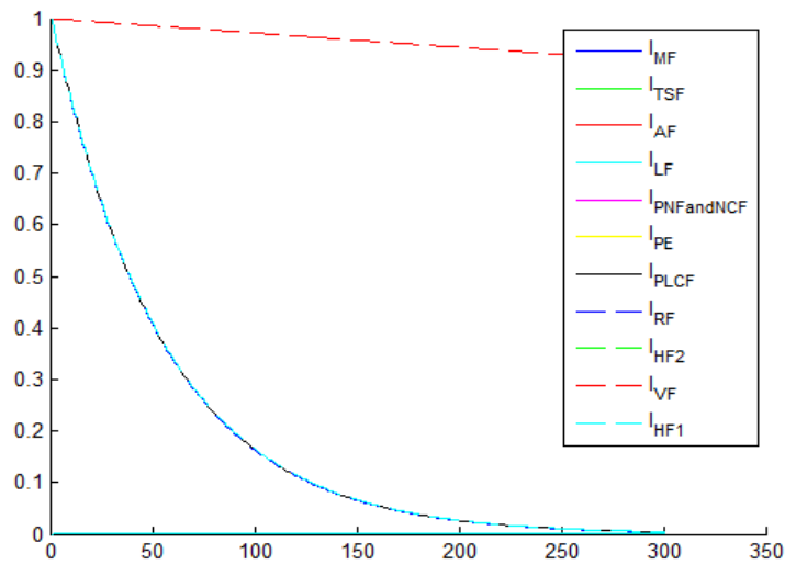
Figure 10. Unreliability of the level crossing system over the time
