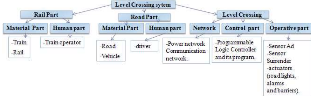
Figure 6. Moroccan Level crossing components
