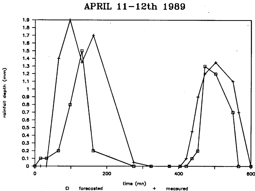
Fig. 13. Rainfall volume for one hour: radar forecast ( \square ) and raingauge measurement ( + ) for April 11-12, 1989.
