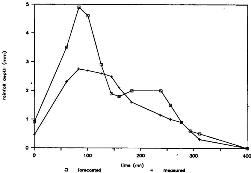
Fig. 14. Rainfall volume for one hour: radar forecast (□) and raingauge measurement (+) for April 27, 1989.
